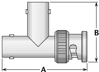
Figure 5 (Tee, jack-jack-plug)
