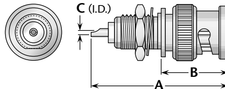
Figure 1 (Front mount)
